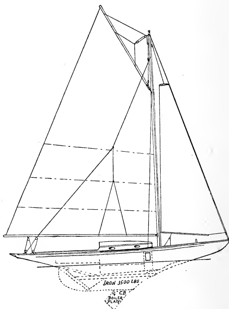
SAIL-PLAN OF SEAWANHAKA KNOCKABOUT— 550 SQUARE FEET.
